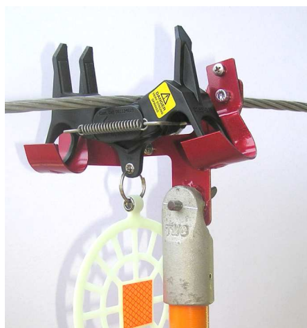
Fitting to overhead wires with application tool
